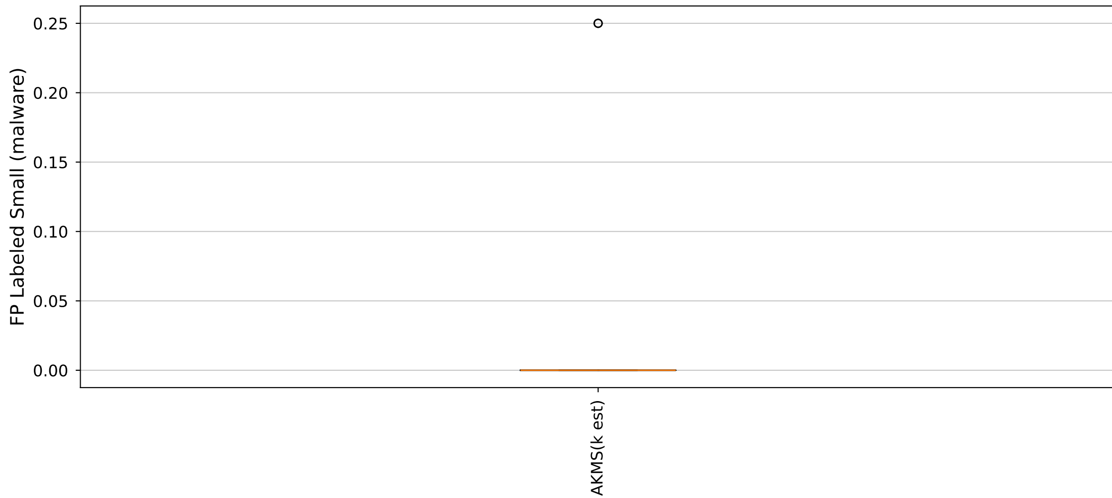
YARA Rules FP Labeled Small (malware) Distribution (Cluster34_Size5 dataset)
